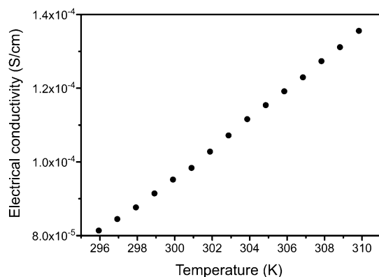
Figure 8. Temperature-activated electrical conduction in a single-crystal device made from Cd 2 (TTFTB).
