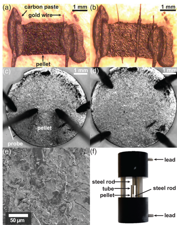
Figure 3. Devices made from \text{Cd}_2(\text{TTFTB}) : (a) A pressed pellet, two-contact probe device made by the wire-paste approach. (b) A pressed pellet, four-contact probe device made by the wire-paste approach. (c) A pressed pellet, four-point probe device made by the direct-contact approach. (d) A pressed pellet, van der Pauw device made by the direct-contact approach. (e) Scanning electron micrograph of a pressed pellet. (f) Home-built apparatus for fabricating and measuring two-contact probe pressed pellet devices in situ.
