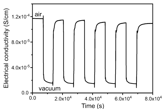
Figure 9. Influence of air and vacuum on the electrical conductivity of single-crystal devices made from Cd 2 (TTFTB).
