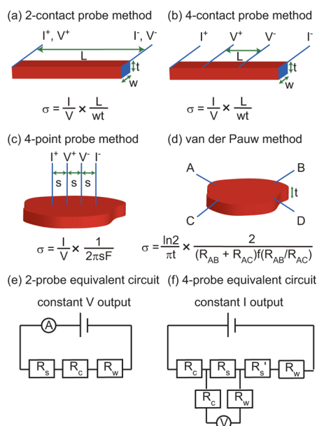
Figure 2. Methods for measuring electrical conductivity of MOFs (a–d). Red and blue areas represent samples and electrodes, respectively. I , current; V , voltage; L , sample length; w , sample width; t , sample thickness; s , distance between adjacent probes; \sigma , electrical conductivity; F and f(R_{AB}/R_{AC}) , correction factors; +, input; –, output. (e) Equivalent circuit for a two-contact probe device. (f) Equivalent circuit for four-contact probe, four-point probe, and van der Pauw devices. R_s , resistance of sample of interest; R_c , contact resistance; R_w , wire resistance; R_s' , sample resistance that is not measured; A, ammeter; V, voltmeter.
