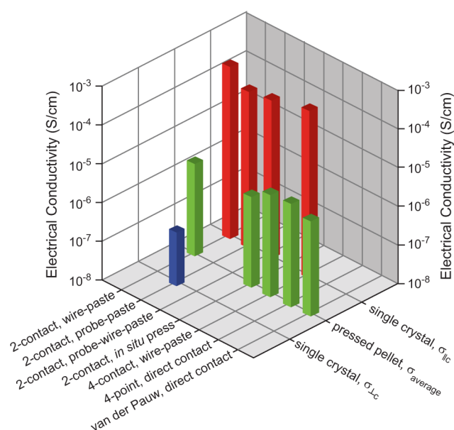
Figure 7. Electrical conductivity data for Cd 2 (TTFTB).
