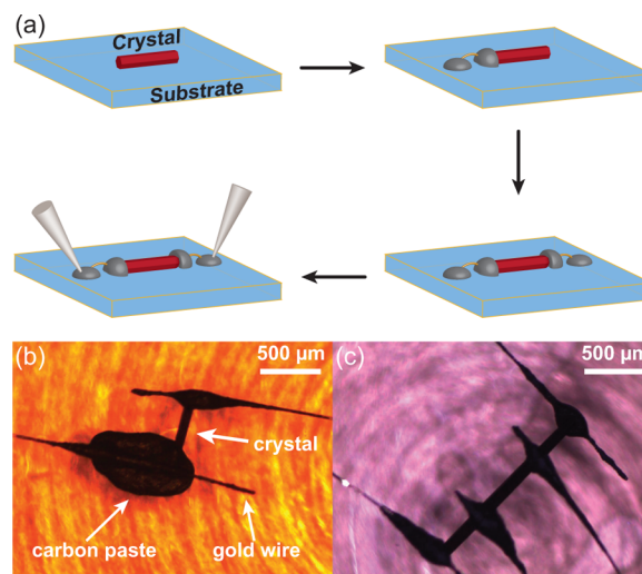
Figure 4. (a) Fabrication scheme of a two-contact probe device made from a single crystal of Cd 2 (TTFTB) using the wire-paste approach. Optical images of two- and four-contact probe single-crystal devices are shown in (b) and (c), respectively.
