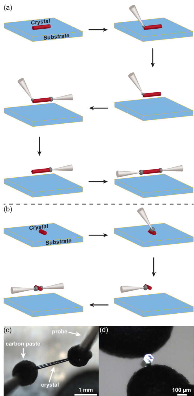
Figure 5. (a,c) Fabrication schematic and optical image of a two-contact probe device made from a single crystal of \text{Cd}_2(\text{TTFTB}) using the probe-paste approach. The electrical conduction was measured parallel to the crystallographic c axis. (b,d) Fabrication schematic and optical image of a two-contact probe device made from a single crystal of \text{Cd}_2(\text{TTFTB}) using the probe-paste approach. The electrical conduction was measured perpendicular to the crystallographic c axis.
