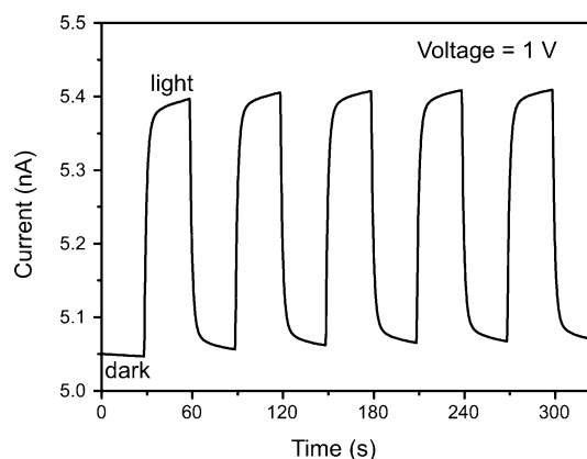
Figure 10. Influence of broadband illumination on the electrical conductivity of a single-crystal device made from Cd 2 (TTFTB).
