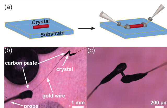
Figure 6. Fabrication schematic and optical images of a two-contact probe device made from a single crystal of \text{Cd}_2(\text{TTFTB}) using the probe-wire-paste approach.
